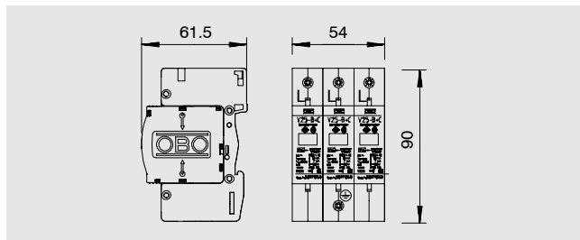
Dimension drawing
