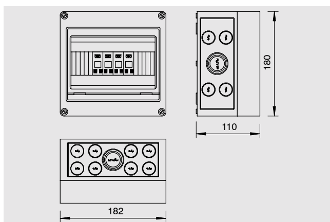
Dimension drawing
